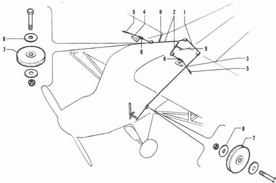
Figure 45. Flap Control System
