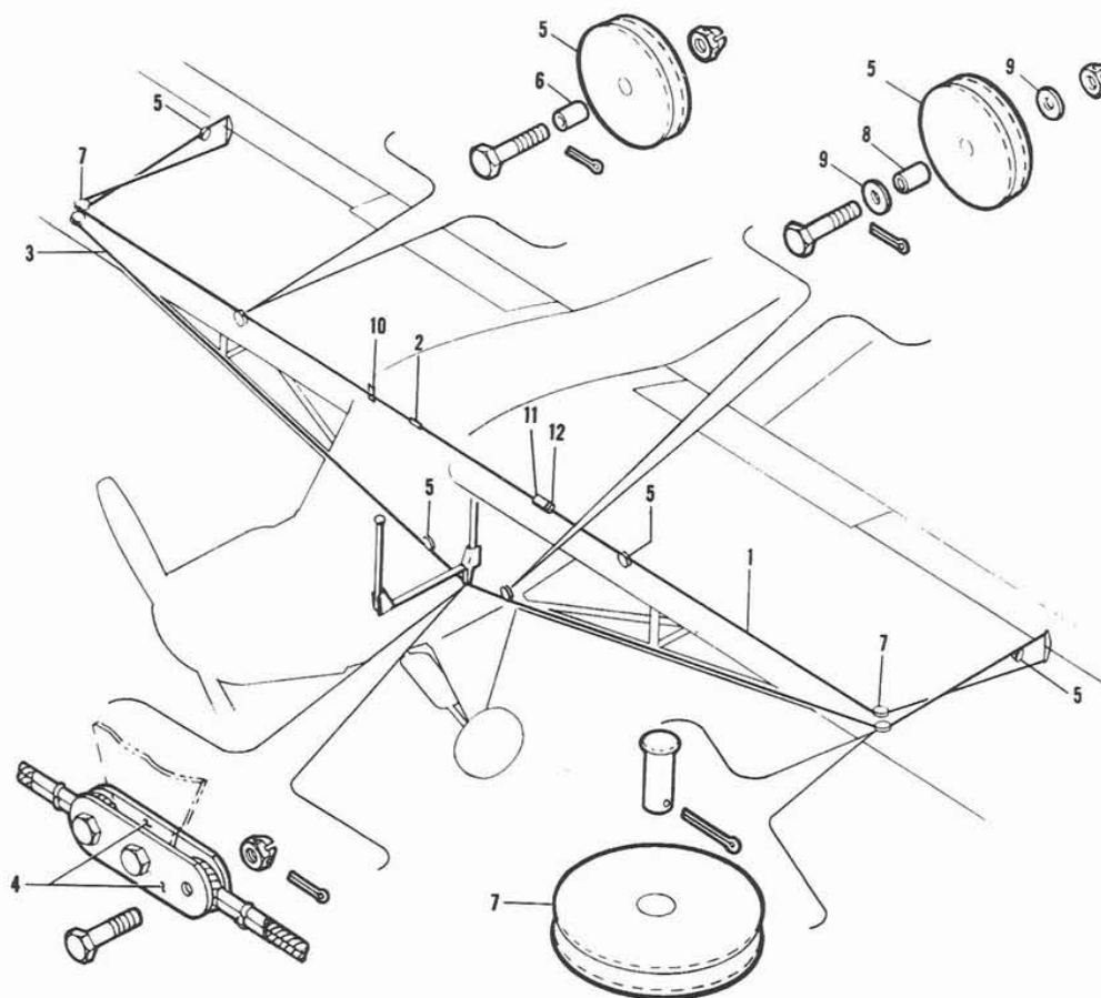
Figure 43. Aileron Control System
