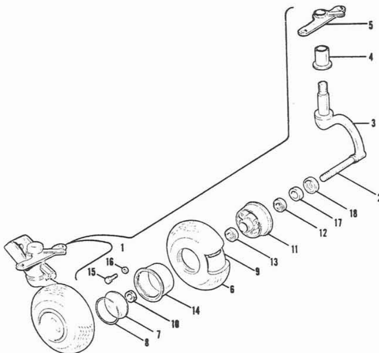
Figure 27A. Tail Wheel Installation 8" Maule
