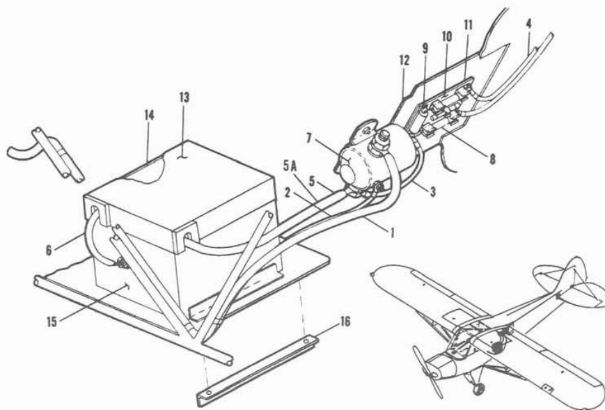
Figure 38. Battery Box Installation
