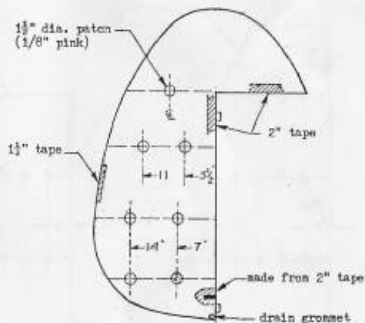
RUDDER p/n 42168
