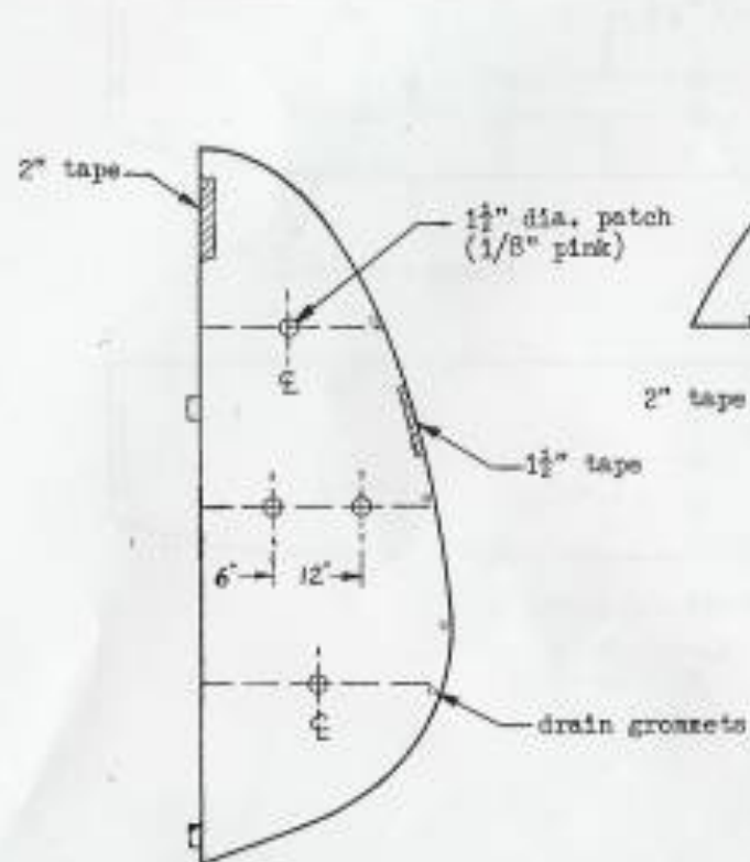
ELEVATOR p/n 41692
