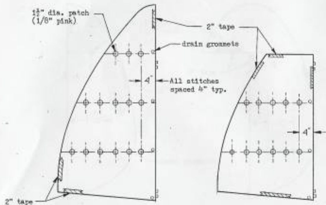
STABILIZER p/n 41652
