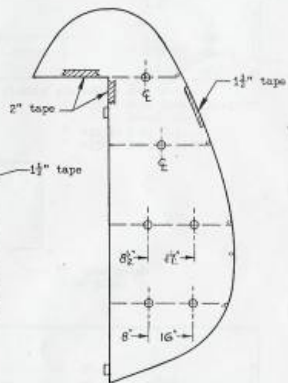
ELEVATOR p/n 12789
