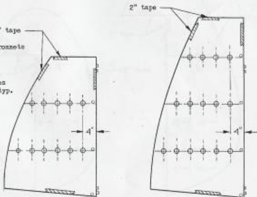
STABILIZER p/n 12648
