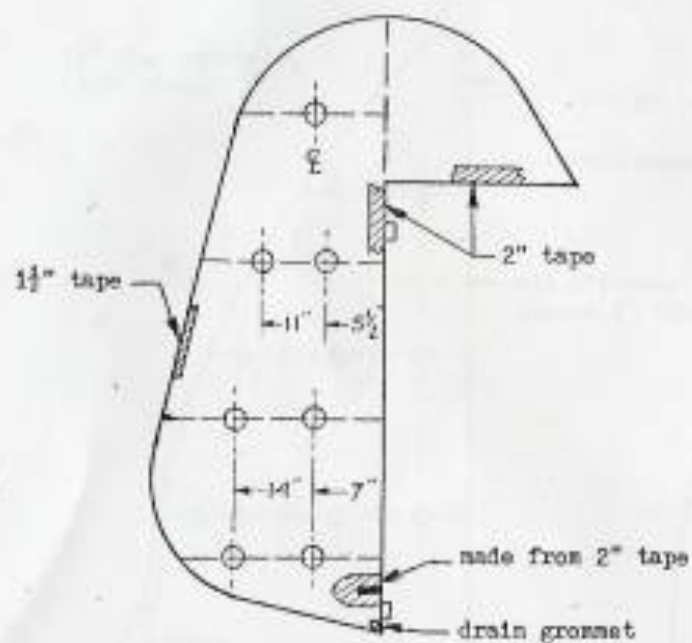
RUDDER p/n 41733
